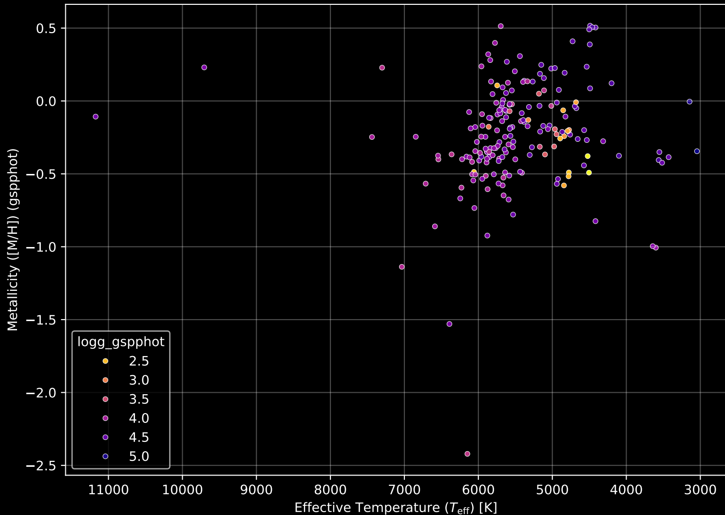
APOGEE DR17 Field: [155+65_MGA] Stellar Population Parameters (n= 190)
