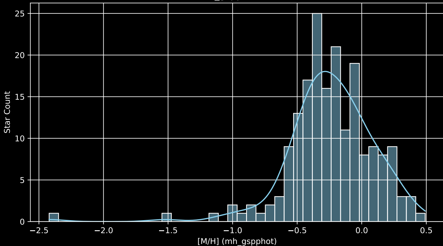
APOGEE DR17 Field: [155+65_MGA [M/H] (mh_gspphot) (n= 186)
