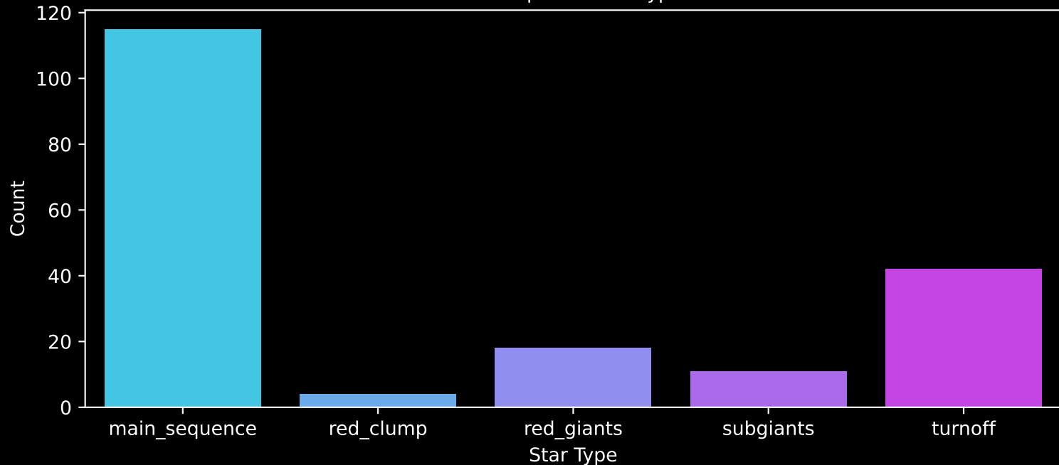
APOGEE DR17 Field: [155+65_MGA] Count plot of Star Type
