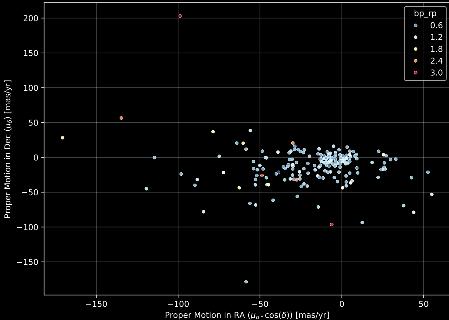
APOGEE DR17 Field: [155+65_MGA] Proper Motion Diagram (n= 190)
