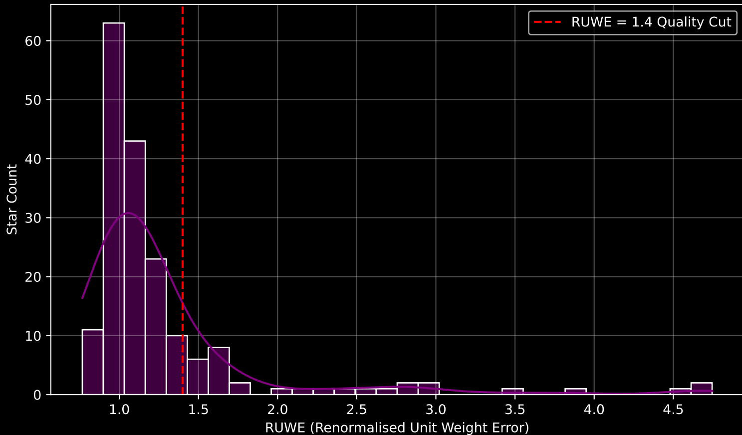
GAPOGEE DR17 Field [155+65_MGA] RUWE Distribution (n= 181)
