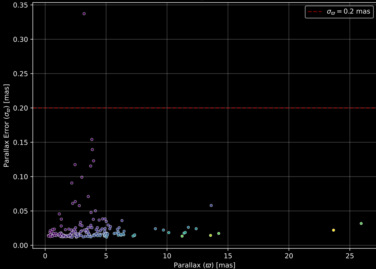
APOGEE DR17 Field: [155+65_MGA] Parallax Quality (n= 190)
